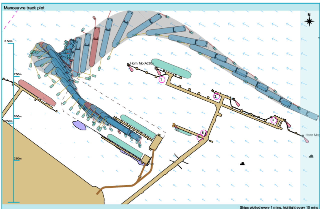
Figure 4.4: Run 19 approach showing preferred swing towards Immingham East and then stern to east
