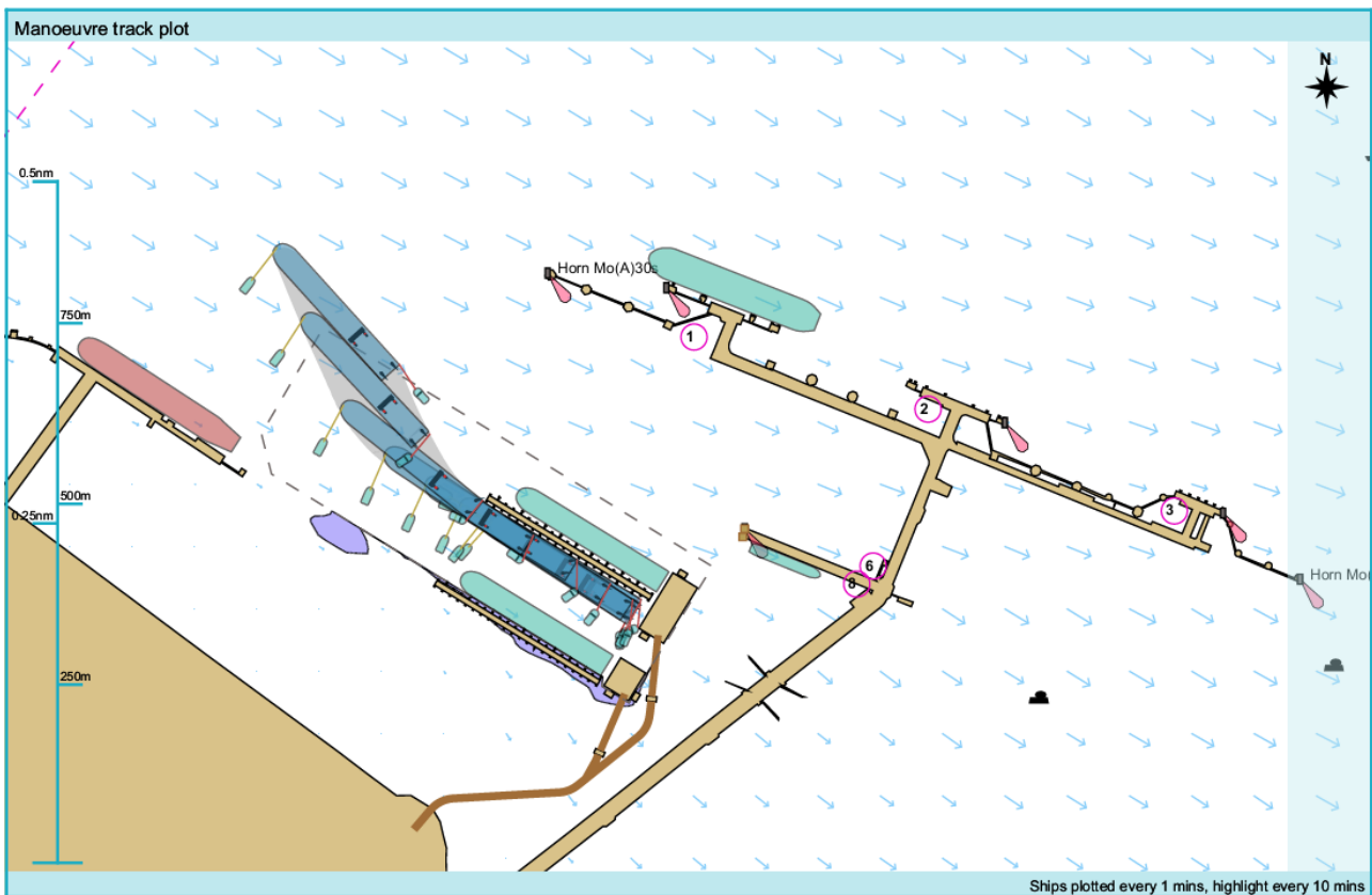
Figure 4.3: Departure using ebb current on port bow to assist departure
