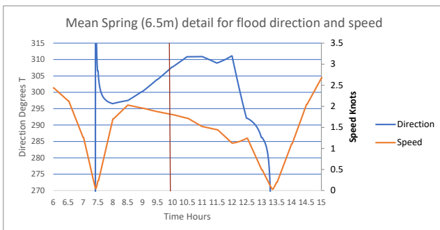
Figure 2.18: Mean spring flood for 7m draught-averaged flow model
