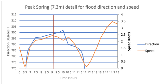
Figure 2.16: Peak spring flood for 7m draught-averaged flow model
