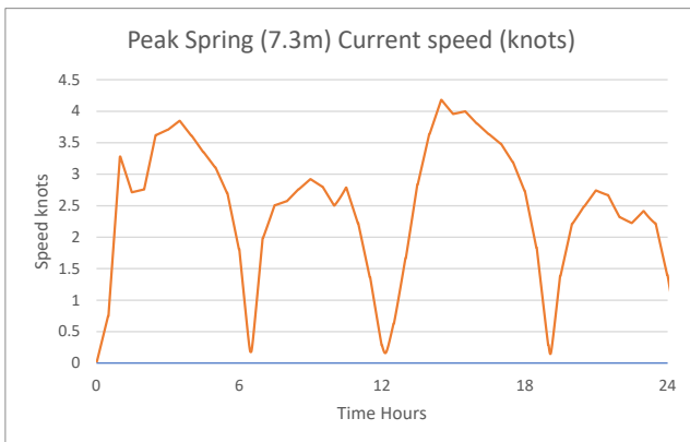
Figure 2.14: Peak spring current speed as simulated
