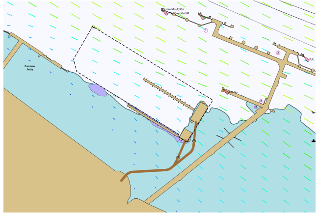
Figure 2.21: Peak spring ebb flows as simulated
