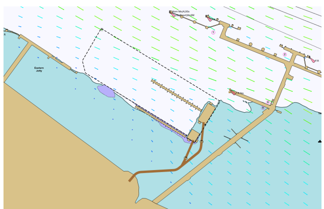
Figure 2.23: Mean spring ebb flows as simulated
