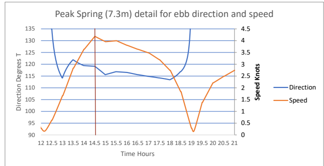
Figure 2.17: Peak spring ebb for 7m draught-averaged flow model
