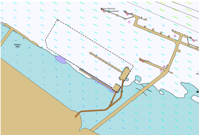
Figure 2.20: Peak spring flood flows as simulated
