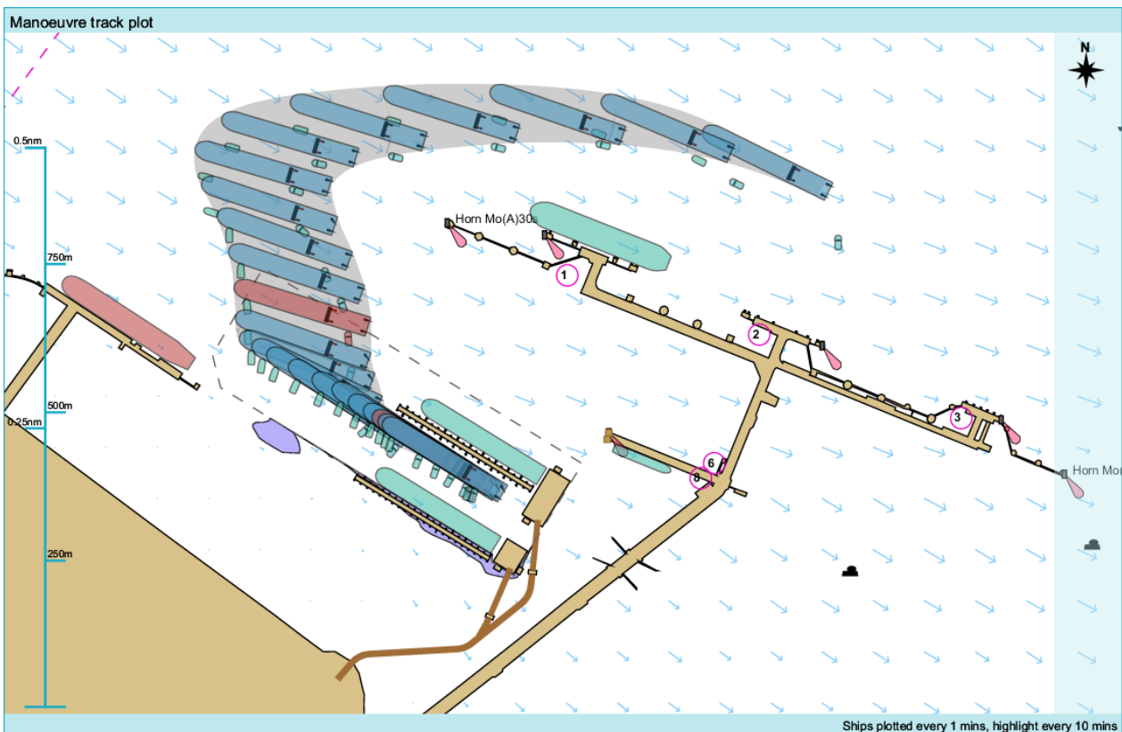
Figure 4.2: Arrival manoeuvre Run 6
