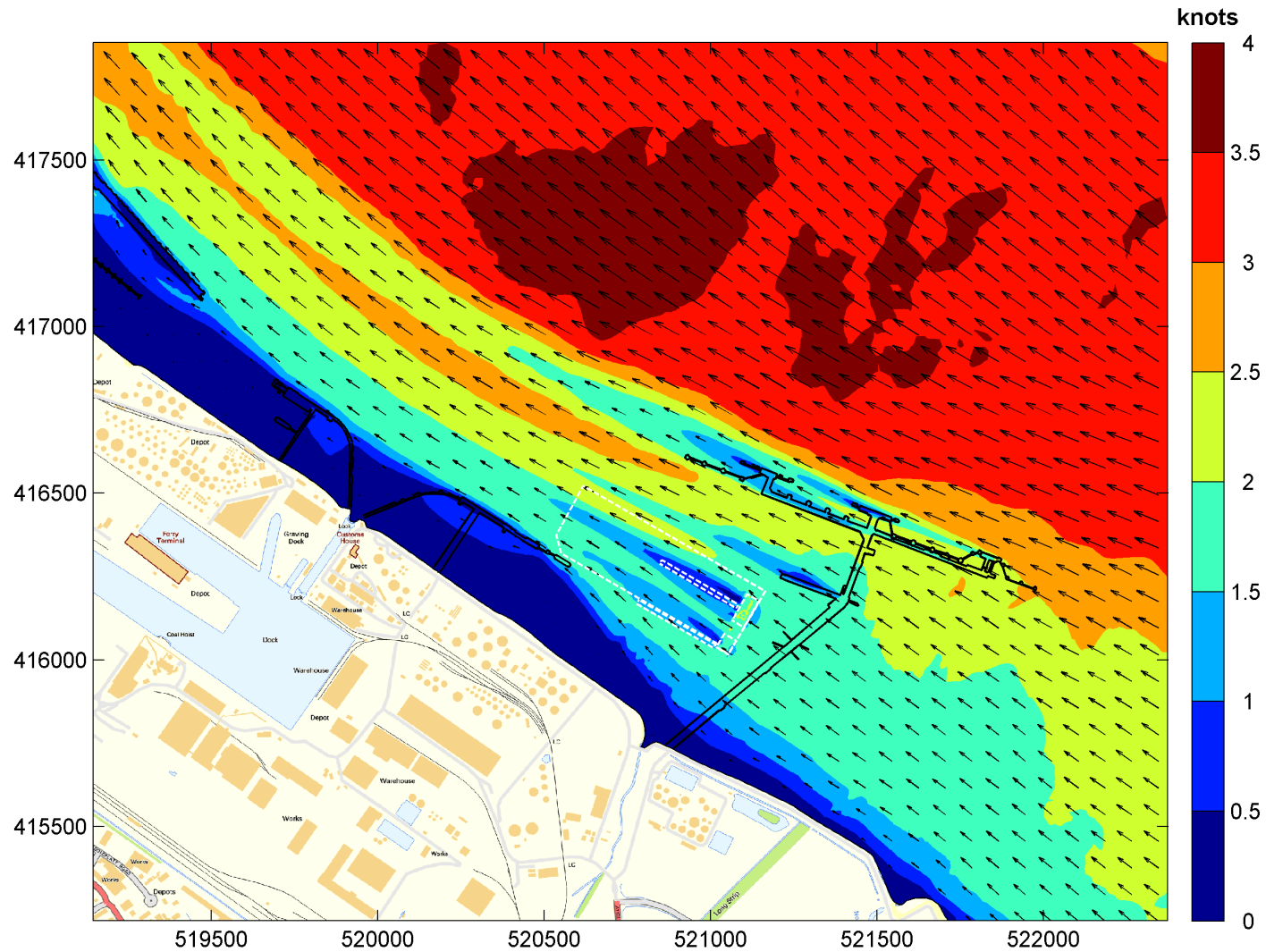
Figure 2.6: Modelled mean spring currents at time of peak flood tide
