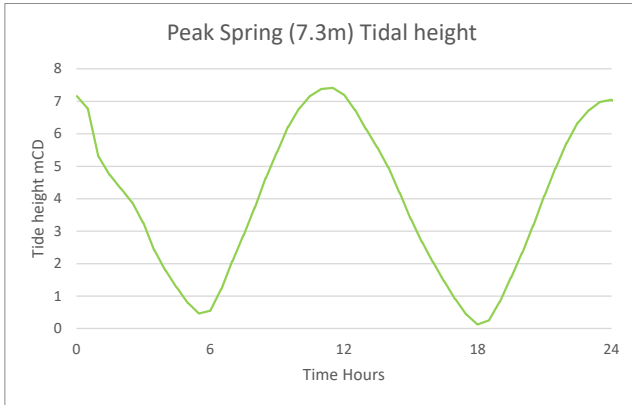
Figure 2.10: Peak spring tidal height as simulated
