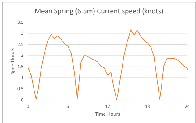
Figure 2.15: Mean spring current speed as simulated
