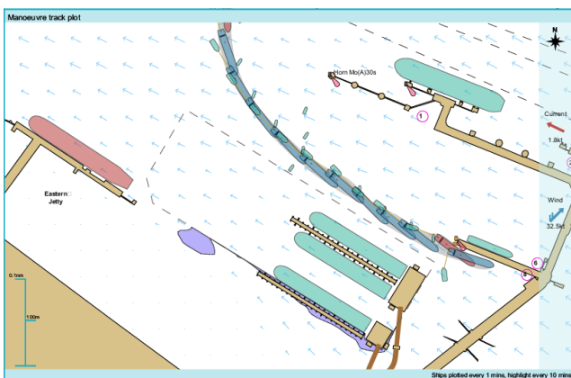
Figure 4.5: Run 42 simulation track plot
