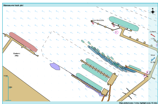
Figure 4.6: Run 52 simulation track plot
