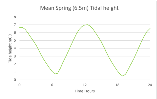
Figure 2.11: Mean spring tidal height as simulated
