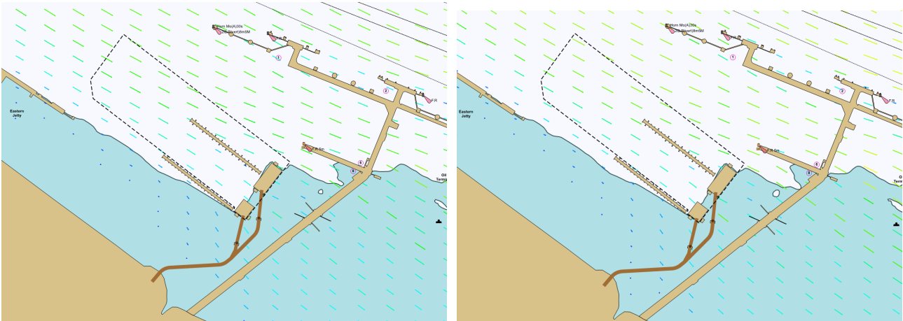
Figure 2.24: Mean spring currents - 306°T orientation Figure 2.25: Peak spring currents - 306°T orientation
